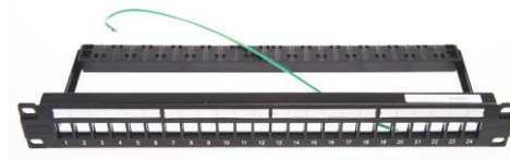
KJX 24 Port Flush Patch Panel
